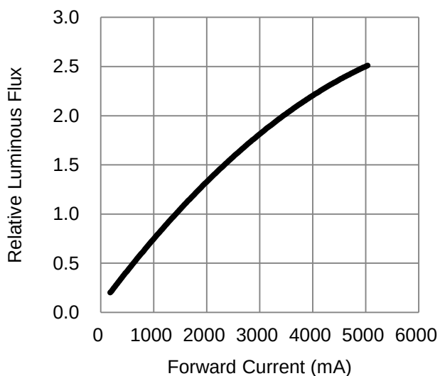
Fig 2. Relative Luminous Flux vs. Forward Current for White at T_c=25 maintained. Do not use below 200mA.
