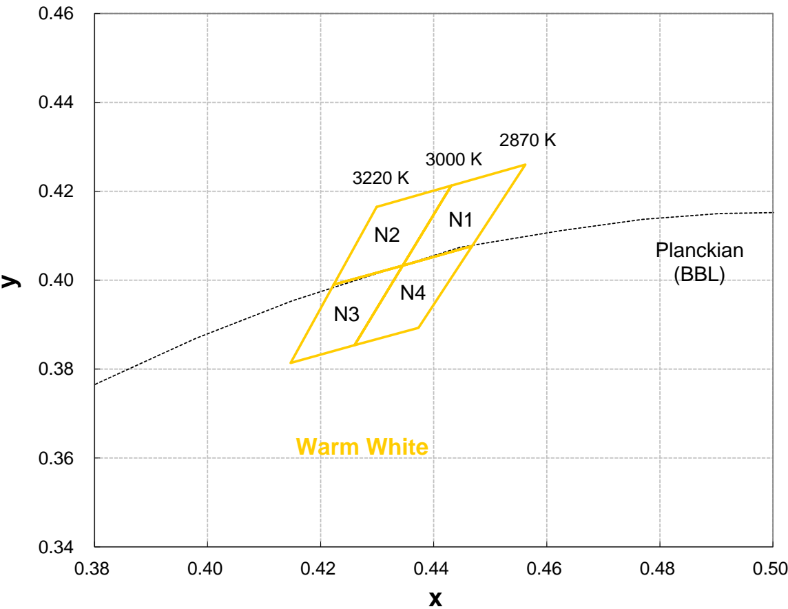
Warm White Binning Structure Graphical Representation
