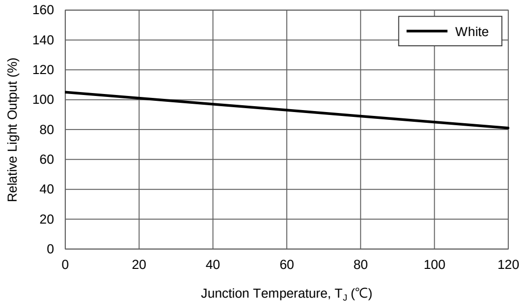
Relative Light Output vs. Junction Temperature at 1750mA
