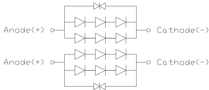
Circuit Diagram
